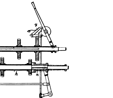
ENGLISH SHOCK REDUCING CHANGE-SPEED MECHANISM.
